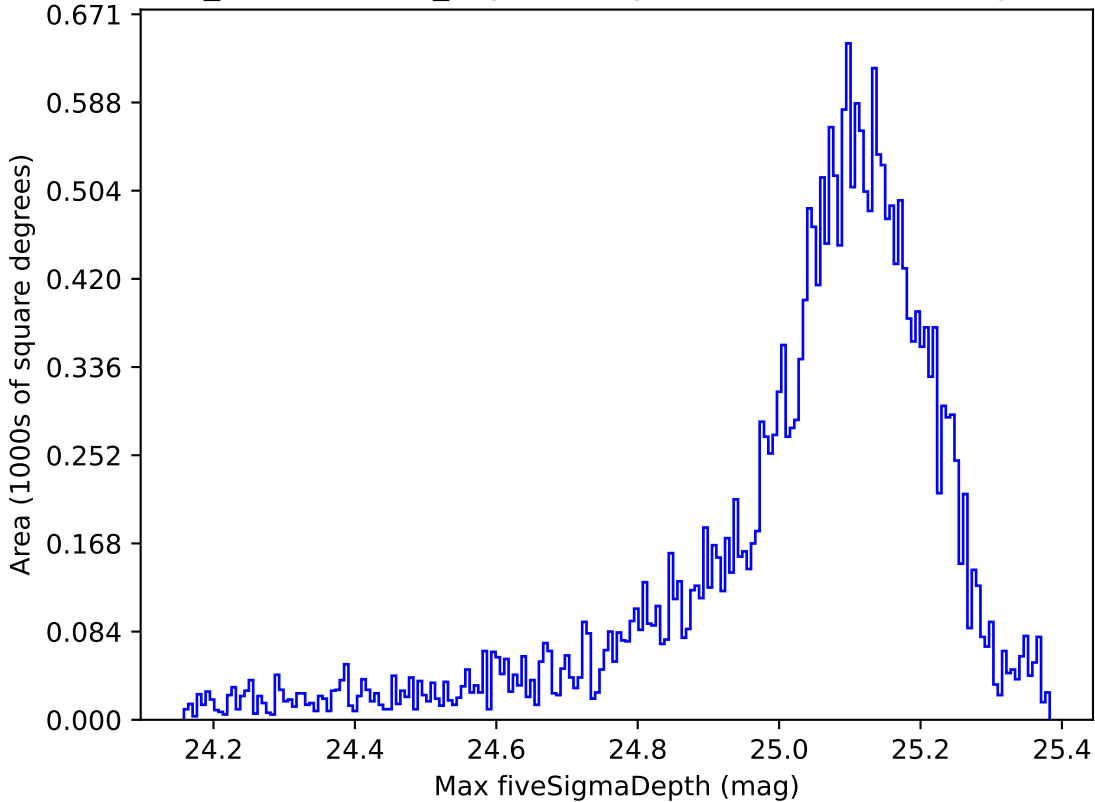
weather_cloudso4v3.4_10yrs All sky all bands: Max fiveSigmaDepth
