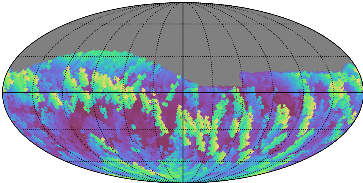
weather_cloudso4v3.4_10yrs Yr 1 z band: Max airmass
