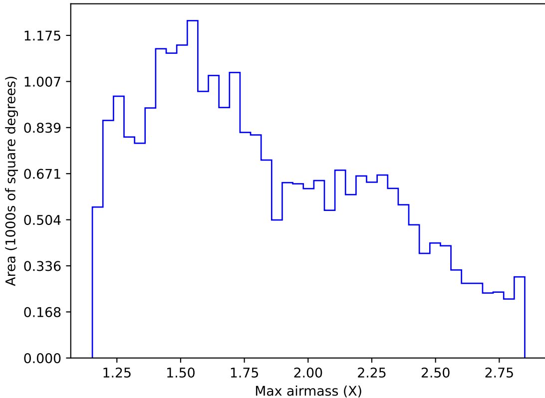
weather_cloudso4v3.4_10yrs Yr 1 z band: Max airmass
