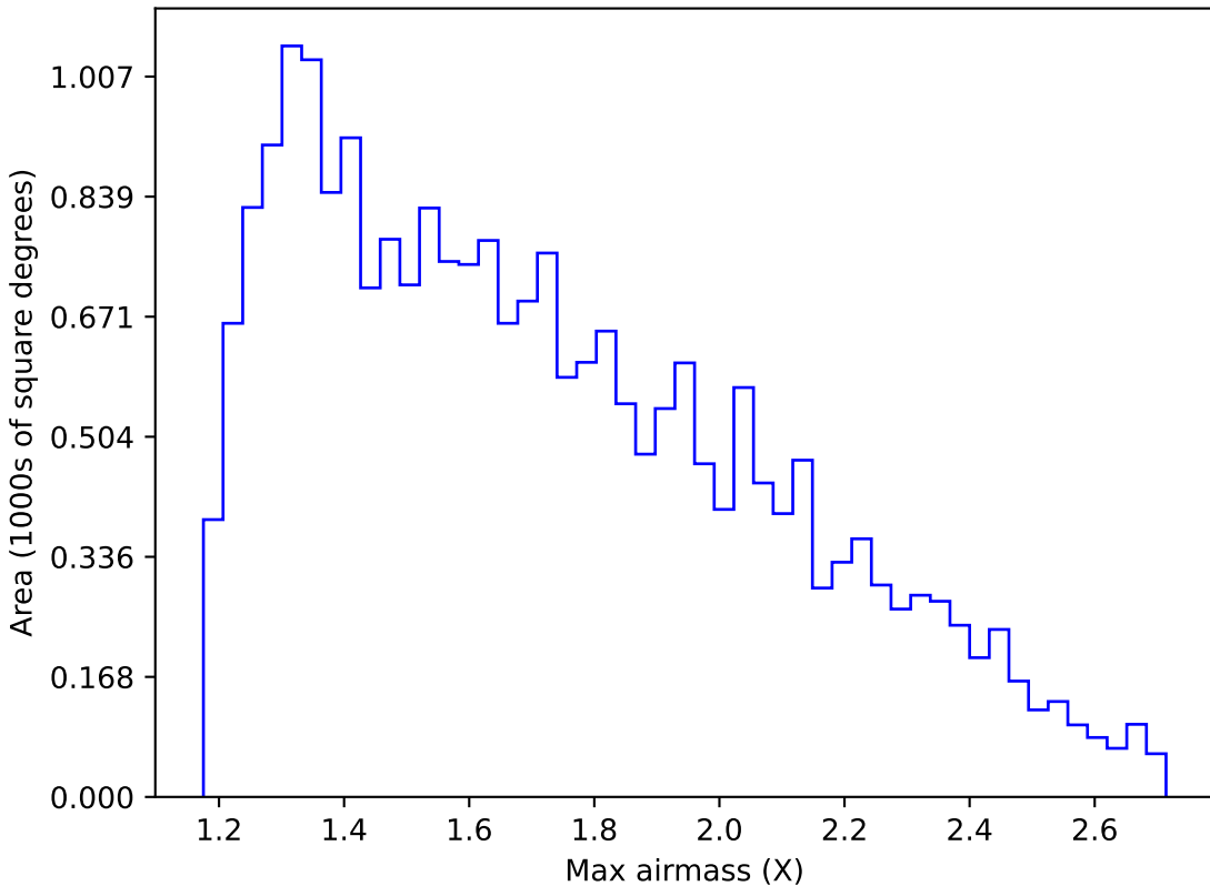
weather_cloudso4v3.4_10yrs Yr 1 y band: Max airmass
