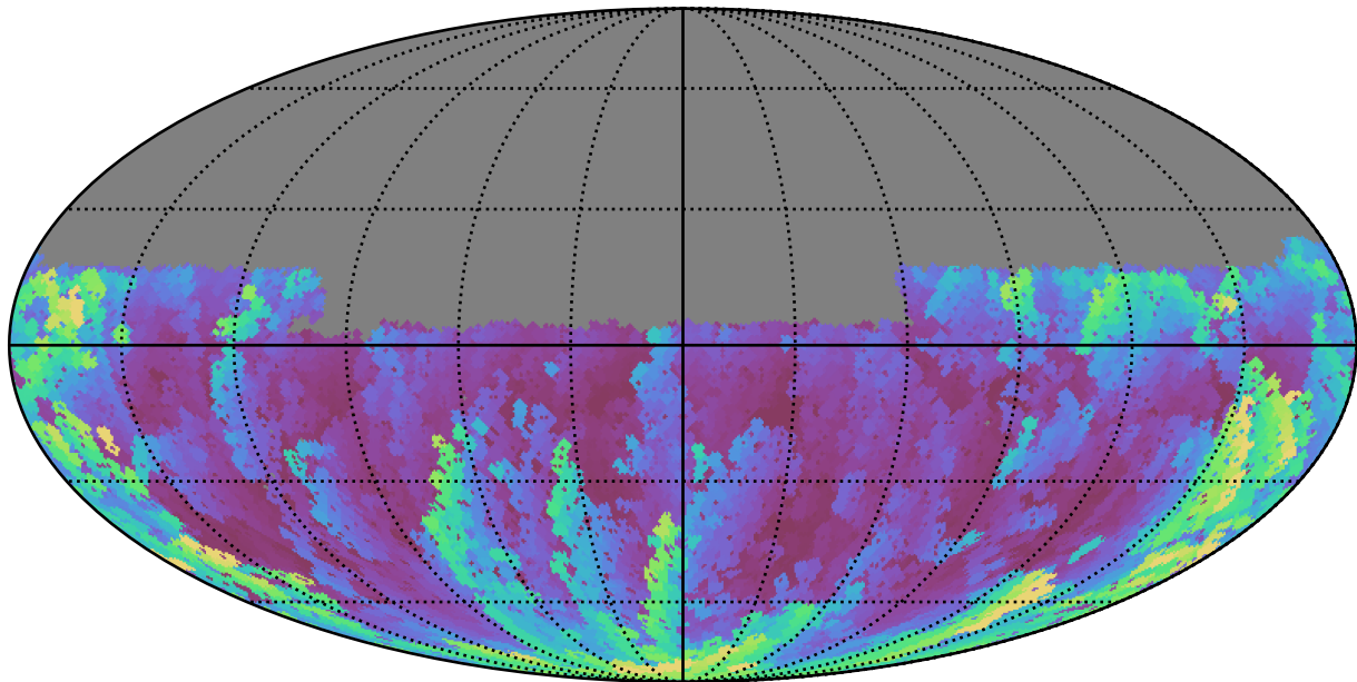
weather_cloudso4v3.4_10yrs Yr 1 u band: Max airmass
