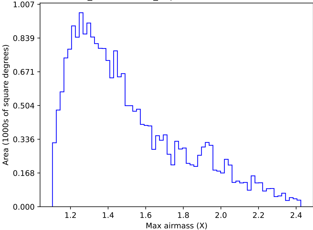
weather_cloudso4v3.4_10yrs Yr 1 u band: Max airmass
