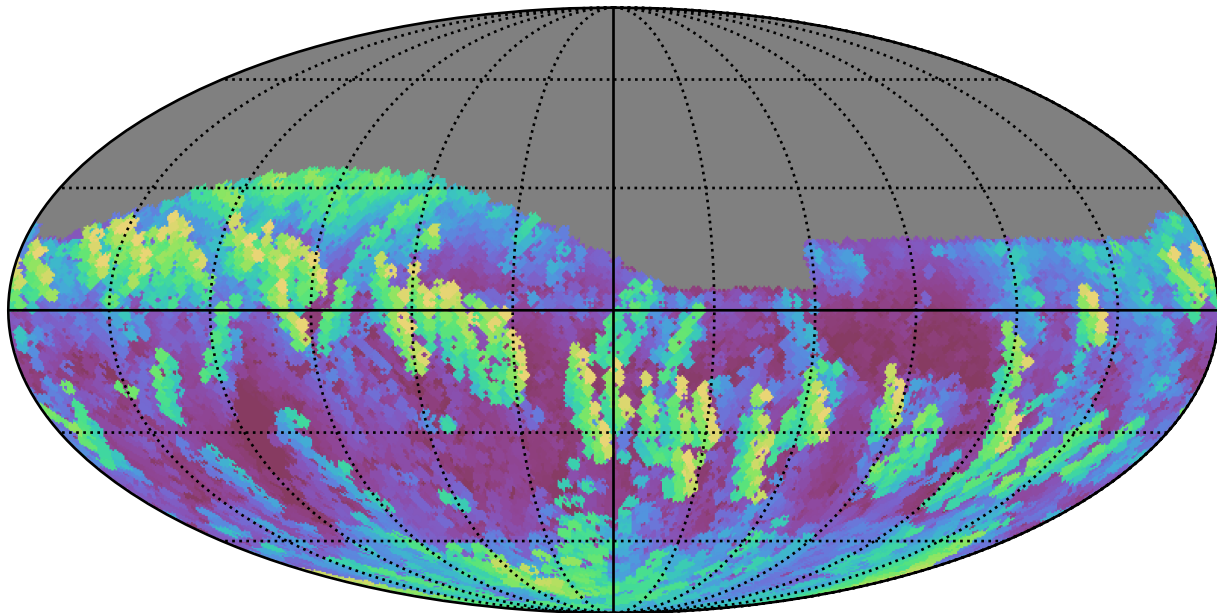
weather_cloudso4v3.4_10yrs Yr 1 i band: Max airmass
