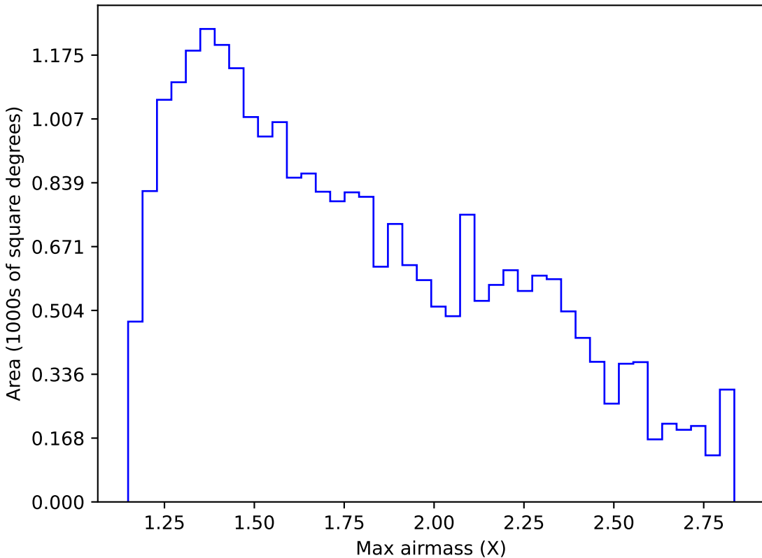
weather_cloudso4v3.4_10yrs Yr 1 i band: Max airmass
