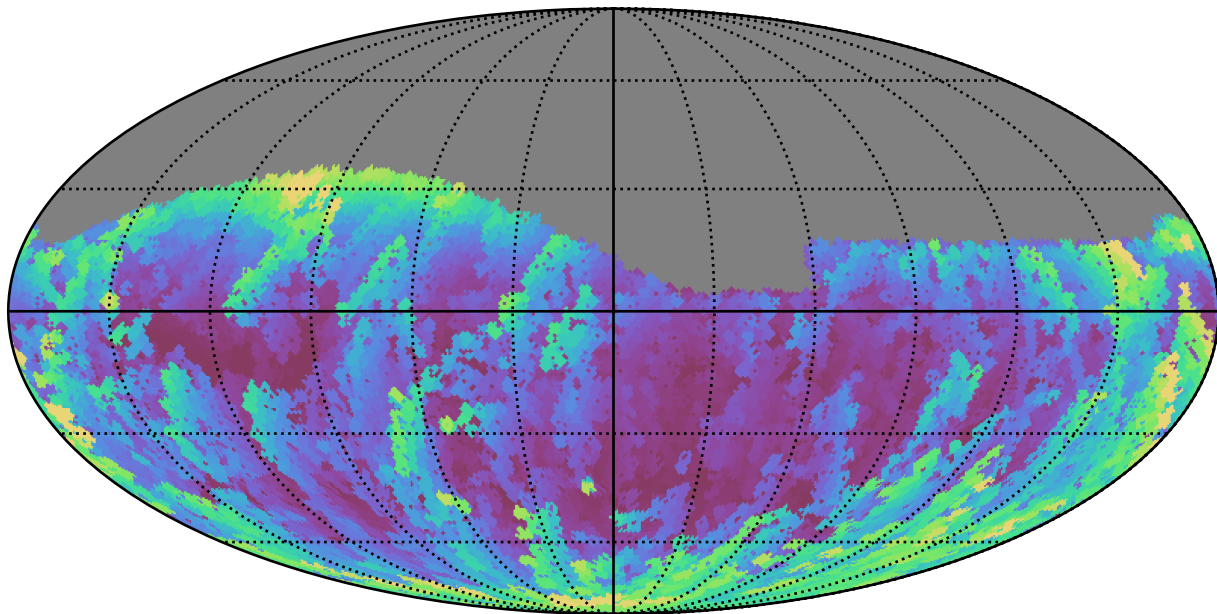
weather_cloudso4v3.4_10yrs Yr 1 g band: Max airmass
