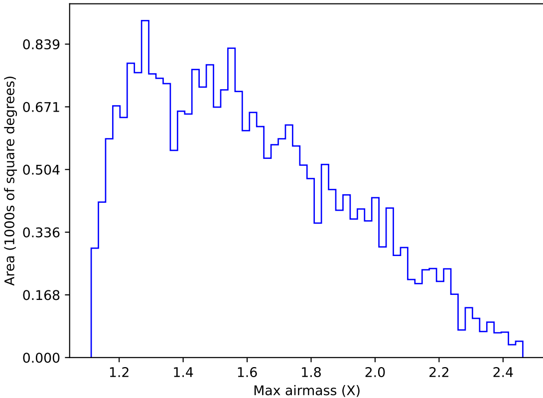
weather_cloudso4v3.4_10yrs Yr 1 g band: Max airmass
