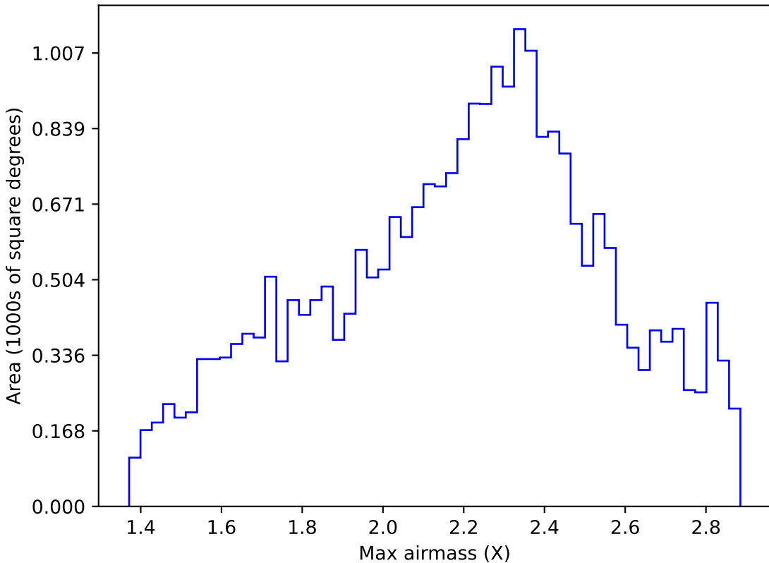
weather_cloudso4v3.4_10yrs Yr 1 all bands: Max airmass
