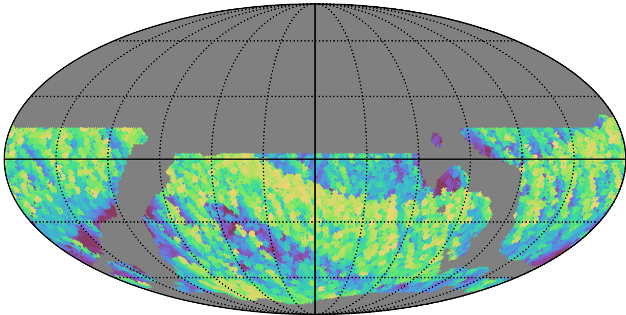
weather_cloudso4v3.4_10yrs WFD z band: Max airmass
