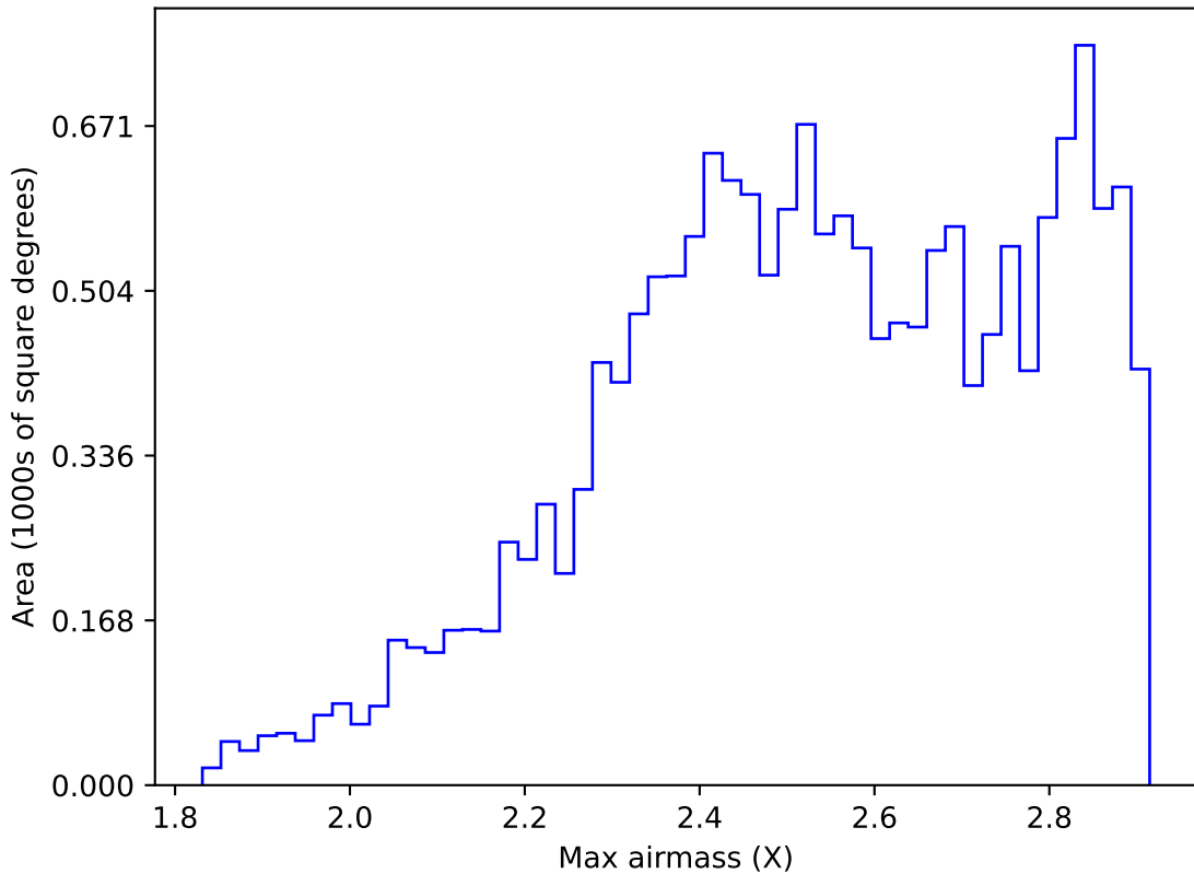
weather_cloudso4v3.4_10yrs WFD z band: Max airmass
