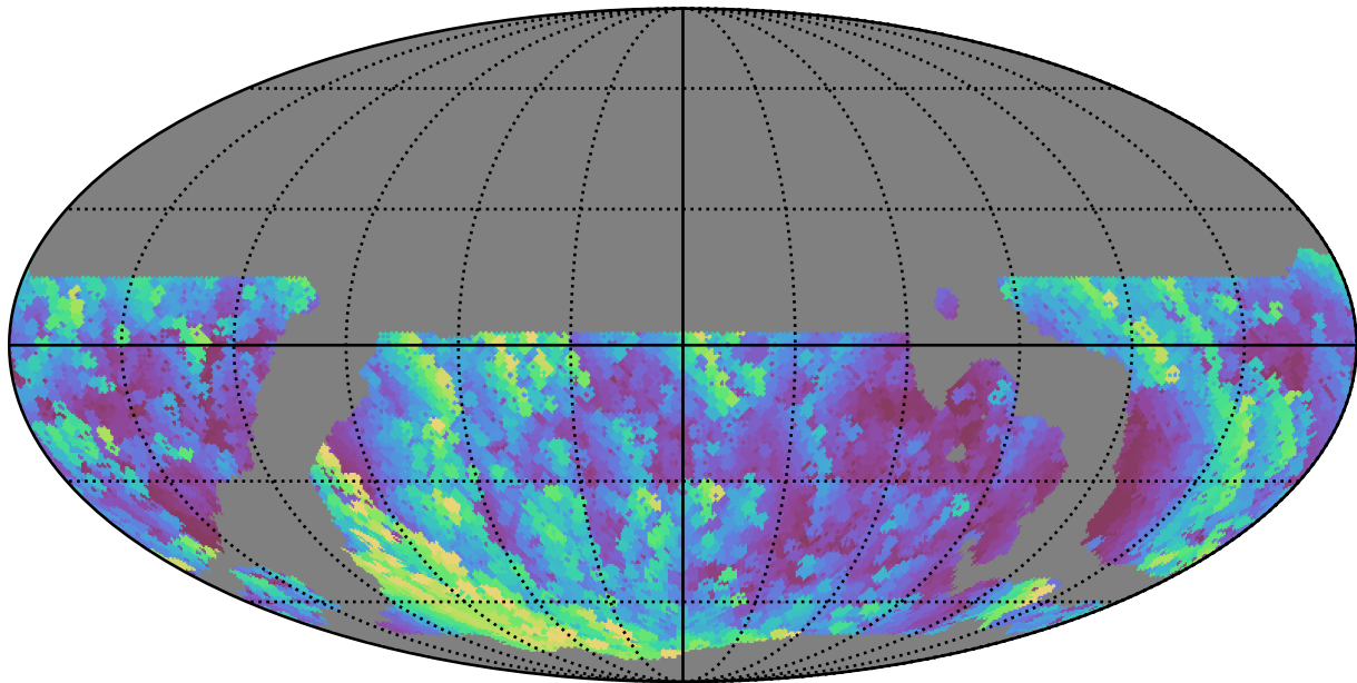
weather_cloudso4v3.4_10yrs WFD u band: Max airmass
