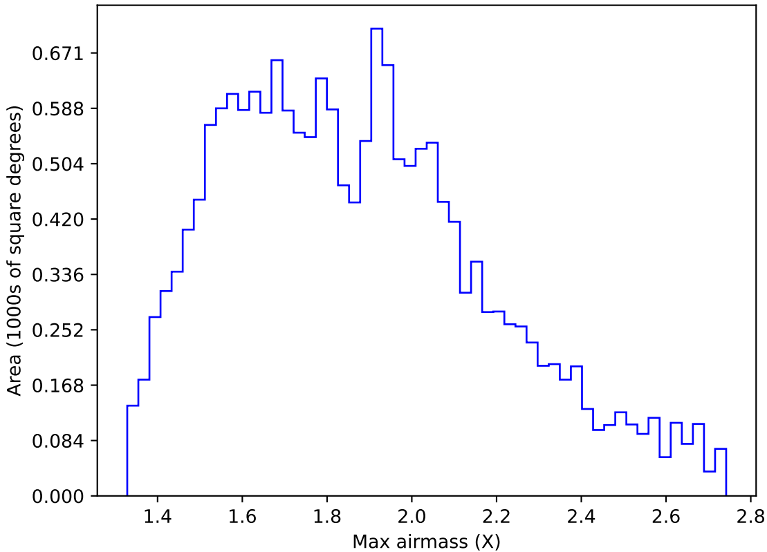
weather_cloudso4v3.4_10yrs WFD u band: Max airmass
