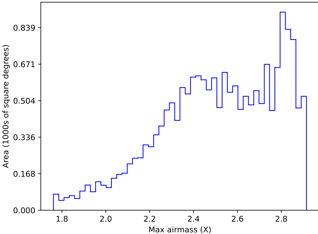
weather_cloudso4v3.4_10yrs WFD i band: Max airmass
