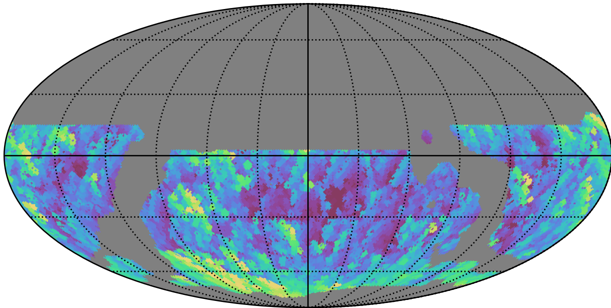
weather_cloudso4v3.4_10yrs WFD g band: Max airmass
