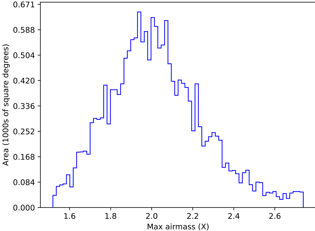
weather_cloudso4v3.4_10yrs WFD g band: Max airmass
