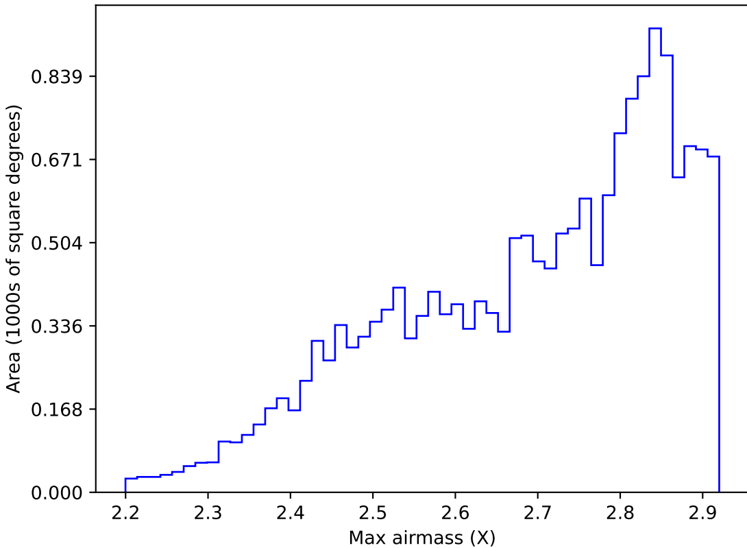
weather_cloudso4v3.4_10yrs WFD all bands: Max airmass
