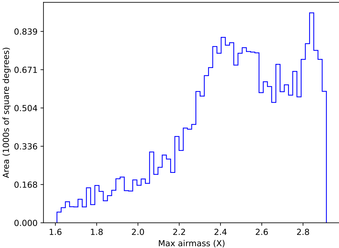
weather_cloudso4v3.4_10yrs All sky z band: Max airmass
