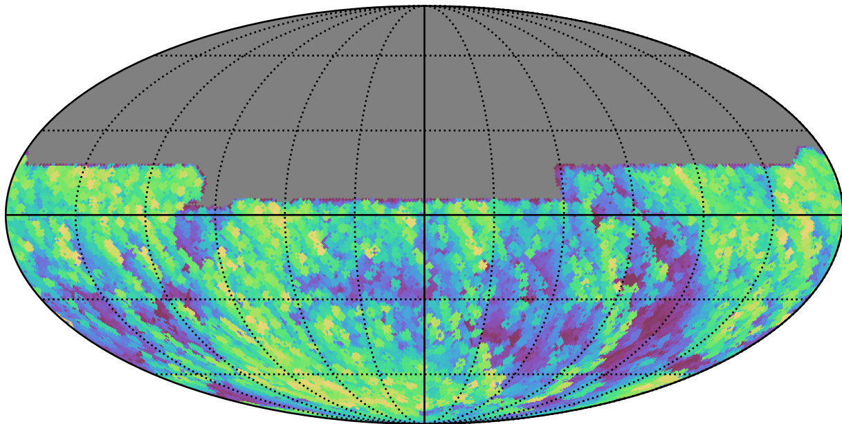
weather_cloudso4v3.4_10yrs All sky y band: Max airmass
