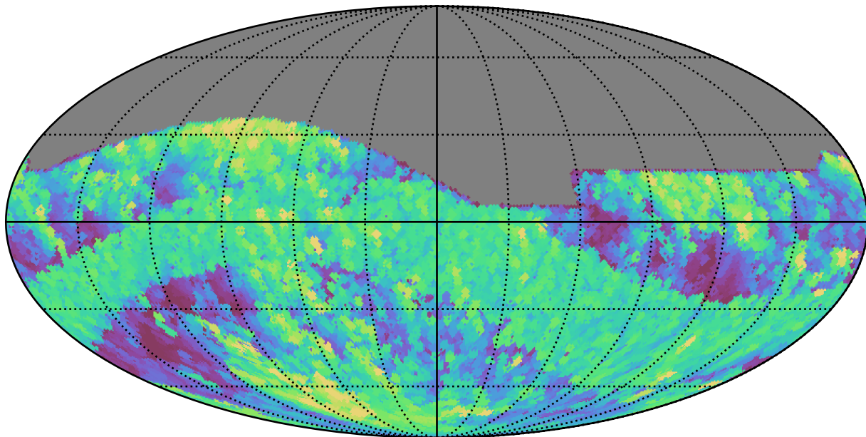
weather_cloudso4v3.4_10yrs All sky r band: Max airmass
