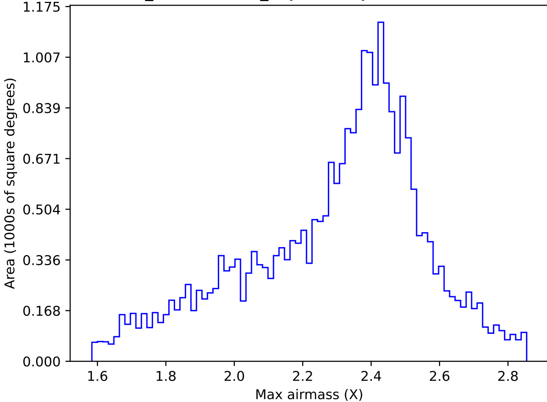
weather_cloudso4v3.4_10yrs All sky r band: Max airmass
