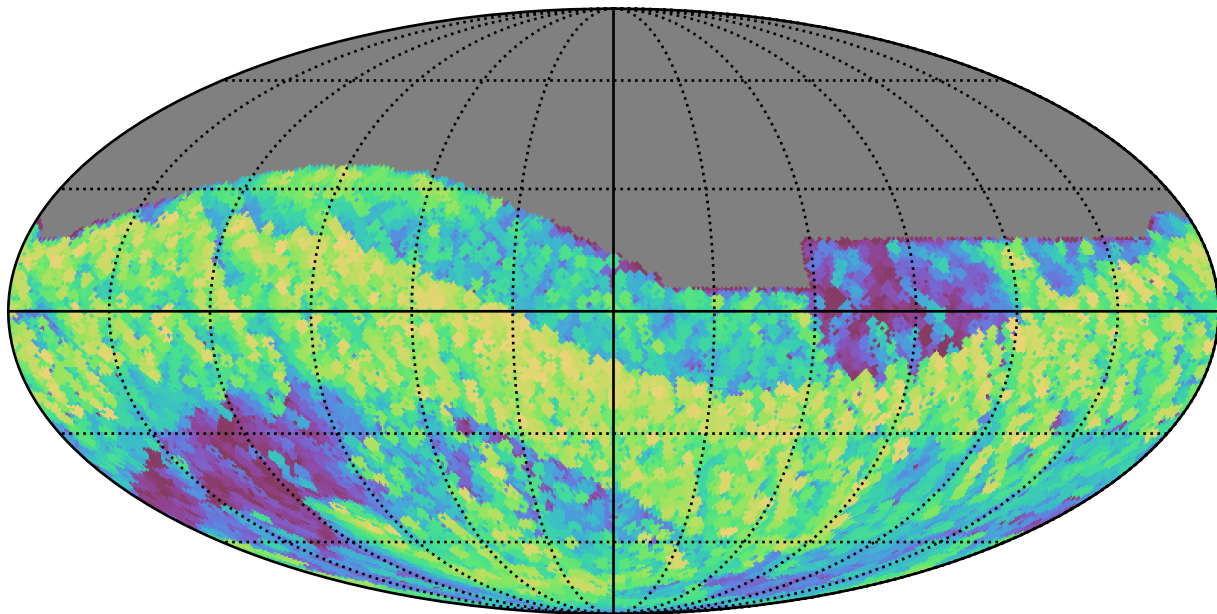
weather_cloudso4v3.4_10yrs All sky i band: Max airmass
