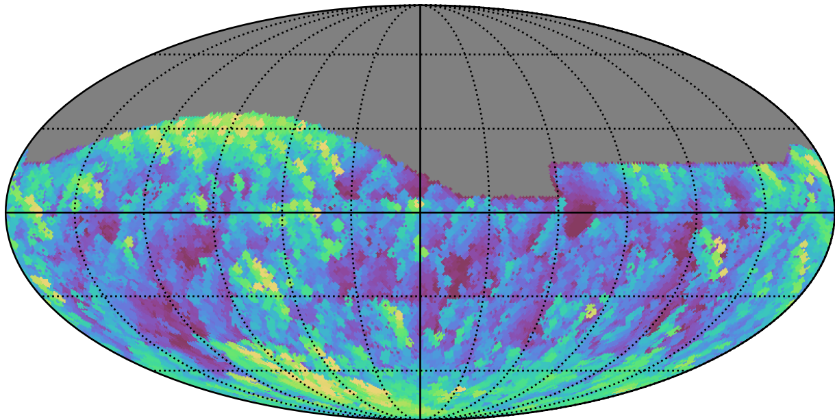
weather_cloudso4v3.4_10yrs All sky g band: Max airmass
