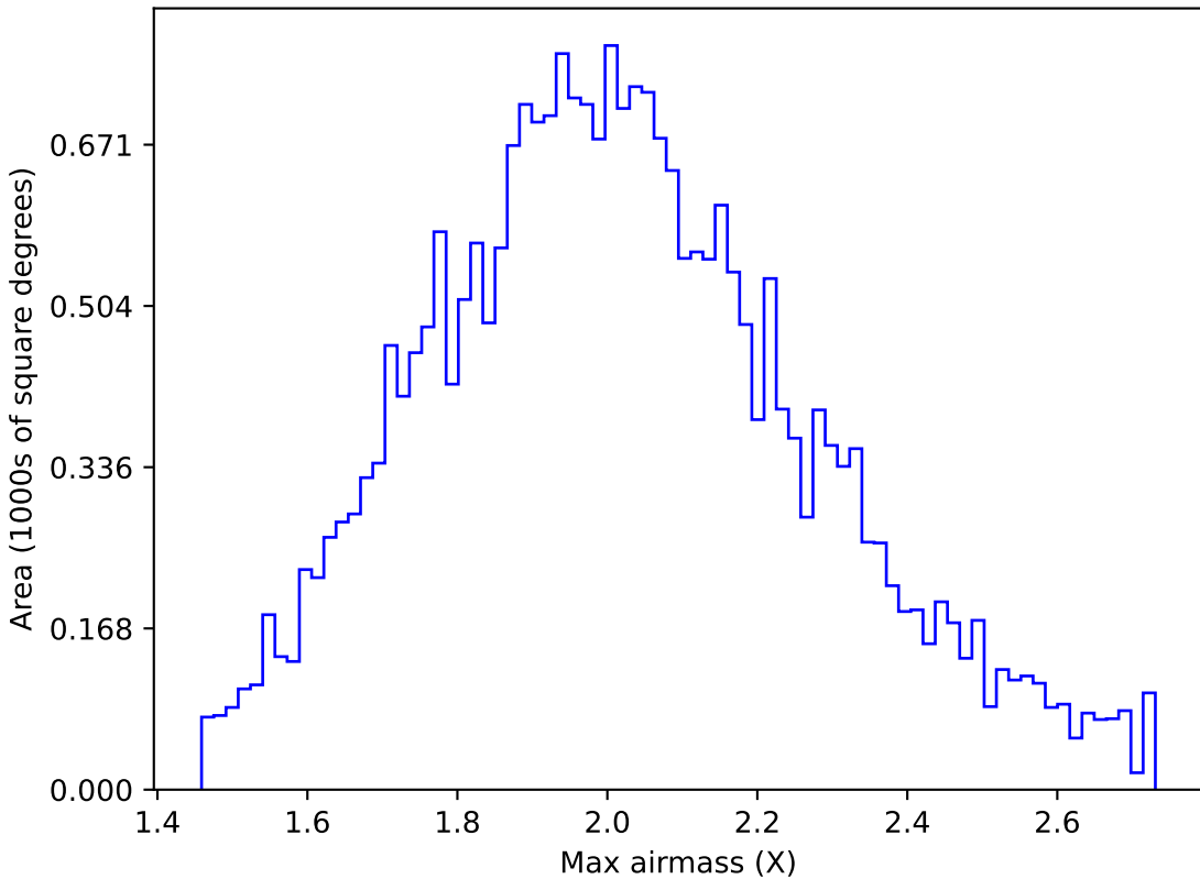
weather_cloudso4v3.4_10yrs All sky g band: Max airmass
