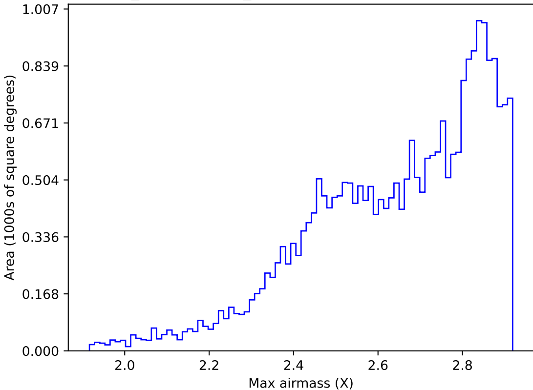
weather_cloudso4v3.4_10yrs All sky all bands: Max airmass
