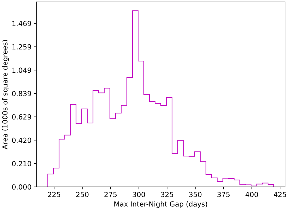
weather_cloudso4v3.4_10yrs WFD z band: Max Inter-Night Gap
