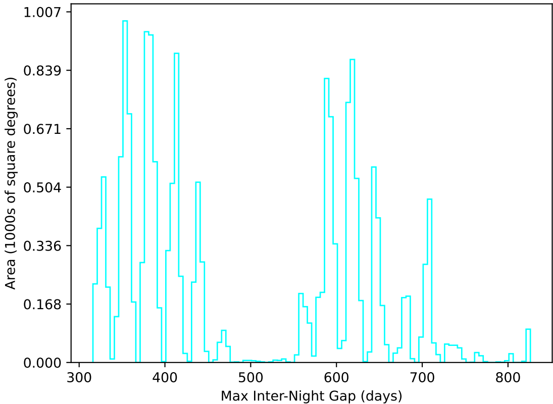
weather_cloudso4v3.4_10yrs WFD u band: Max Inter-Night Gap
