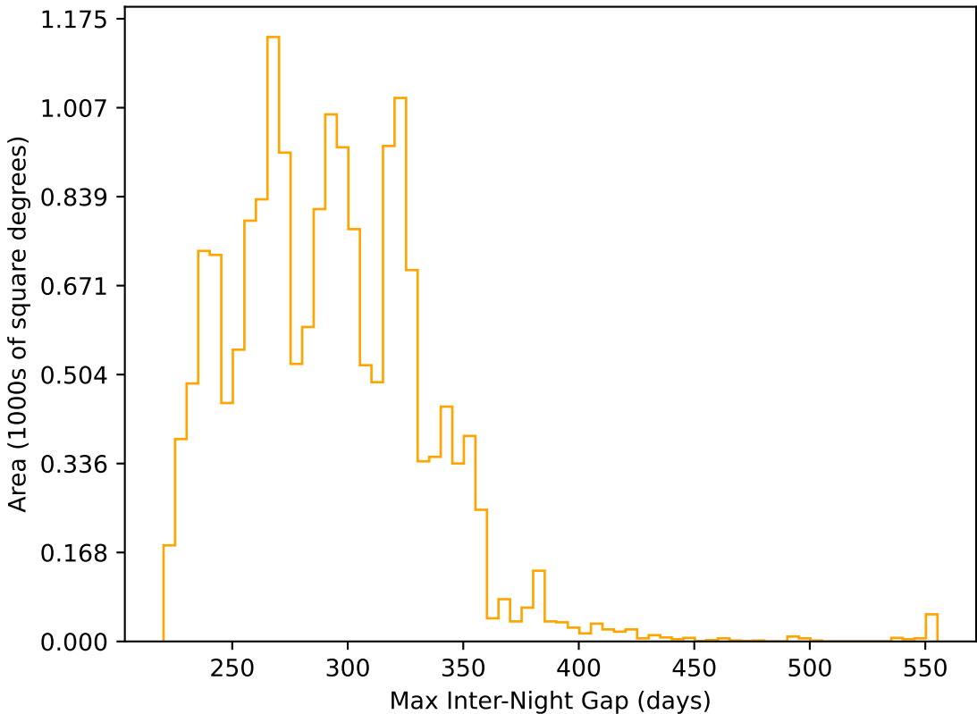
weather_cloudso4v3.4_10yrs WFD r band: Max Inter-Night Gap
