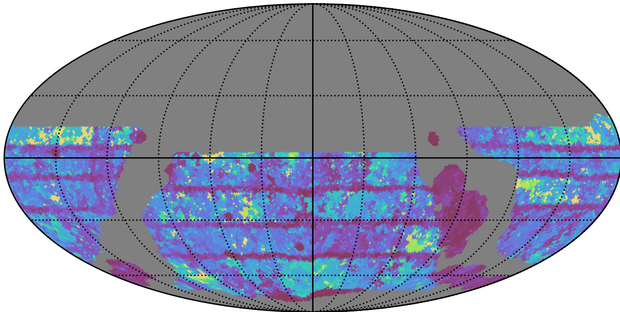
weather_cloudso4v3.4_10yrs WFD i band: Max Inter-Night Gap
