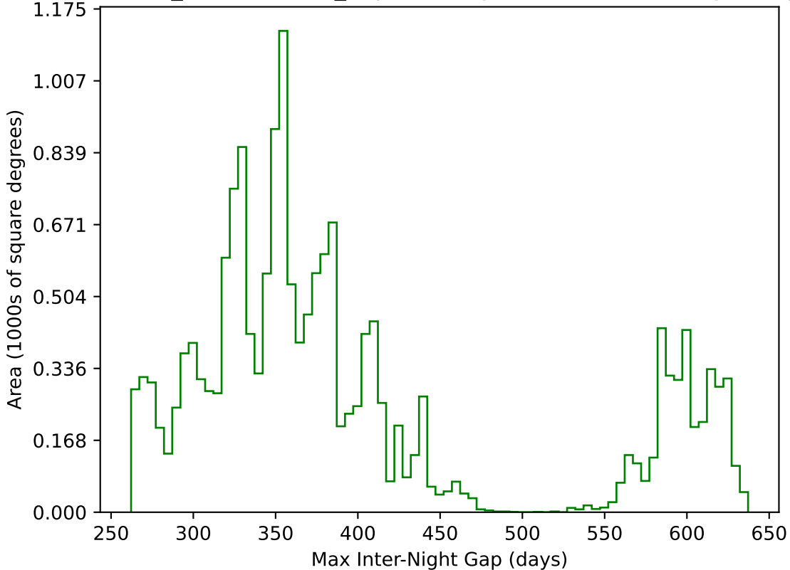
weather_cloudso4v3.4_10yrs WFD g band: Max Inter-Night Gap
