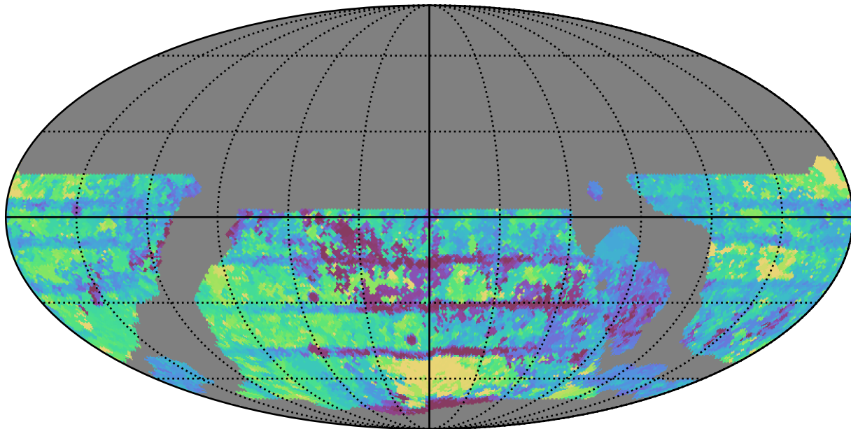
weather_cloudso4v3.4_10yrs WFD all bands: Max Inter-Night Gap
