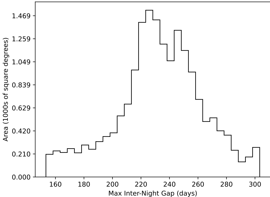
weather_cloudso4v3.4_10yrs WFD all bands: Max Inter-Night Gap
