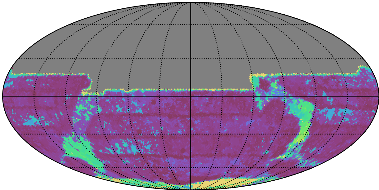
weather_cloudso4v3.4_10yrs All sky y band: Max Inter-Night Gap
