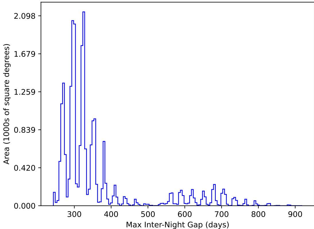
weather_cloudso4v3.4_10yrs All sky y band: Max Inter-Night Gap
