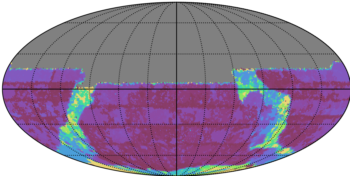
weather_cloudso4v3.4_10yrs All sky u band: Max Inter-Night Gap
