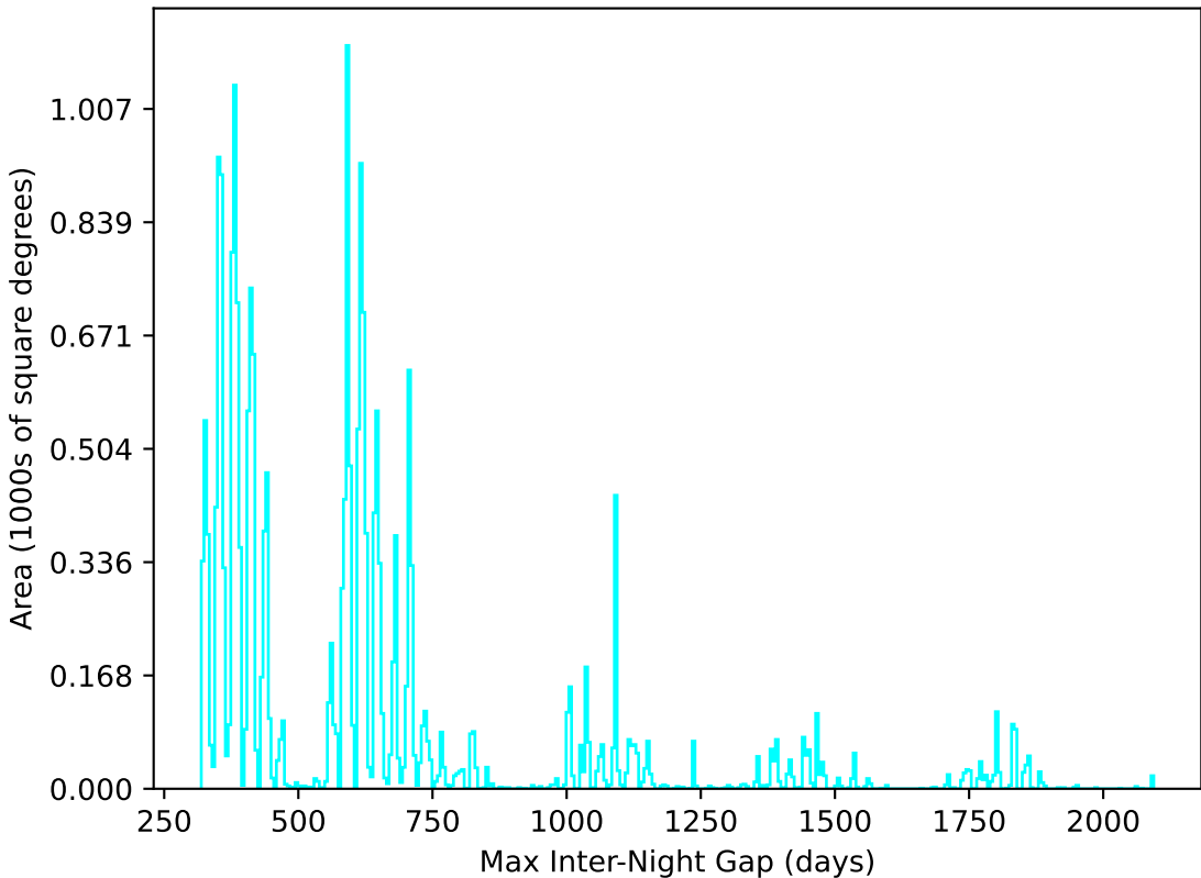
weather_cloudso4v3.4_10yrs All sky u band: Max Inter-Night Gap
