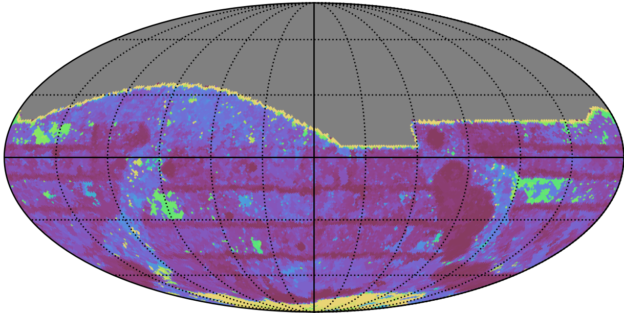
weather_cloudso4v3.4_10yrs All sky r band: Max Inter-Night Gap
