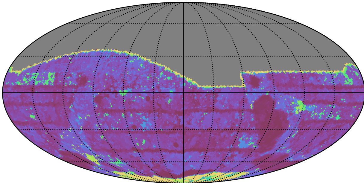
weather_cloudso4v3.4_10yrs All sky i band: Max Inter-Night Gap
