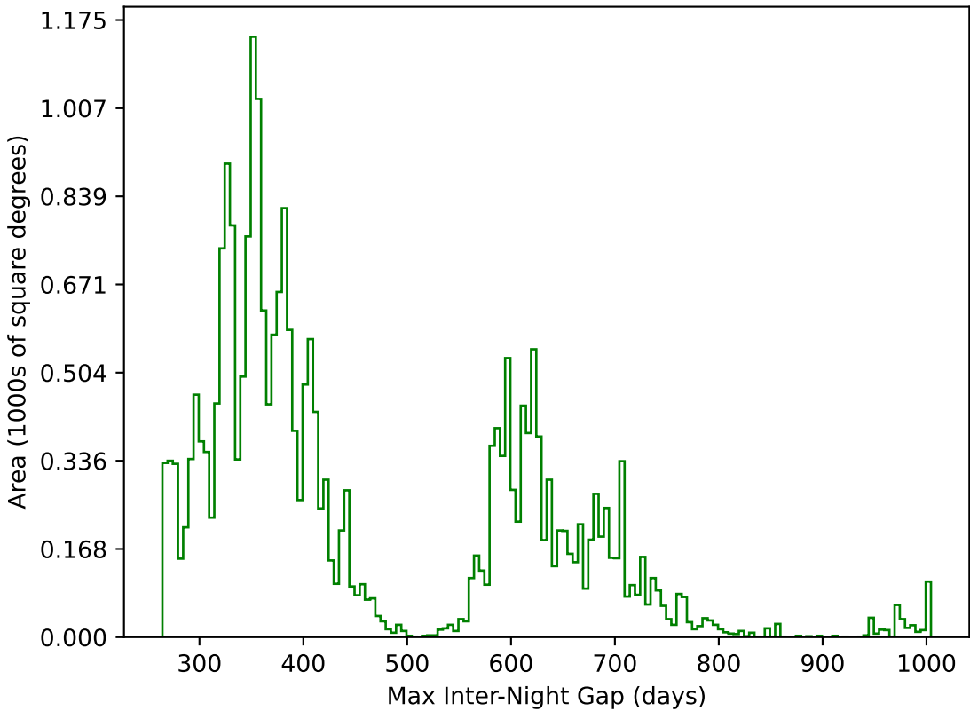
weather_cloudso4v3.4_10yrs All sky g band: Max Inter-Night Gap
