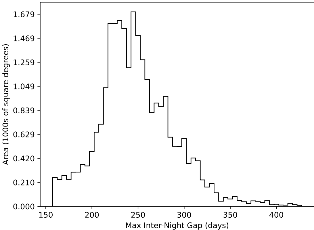
weather_cloudso4v3.4_10yrs All sky all bands: Max Inter-Night Gap
