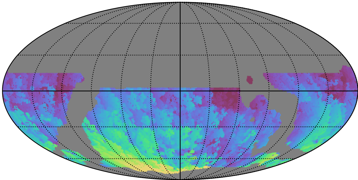
weather_cloudso4v3.4_10yrs WFD u band: Max HA
