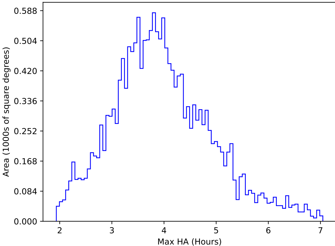
weather_cloudso4v3.4_10yrs WFD u band: Max HA
