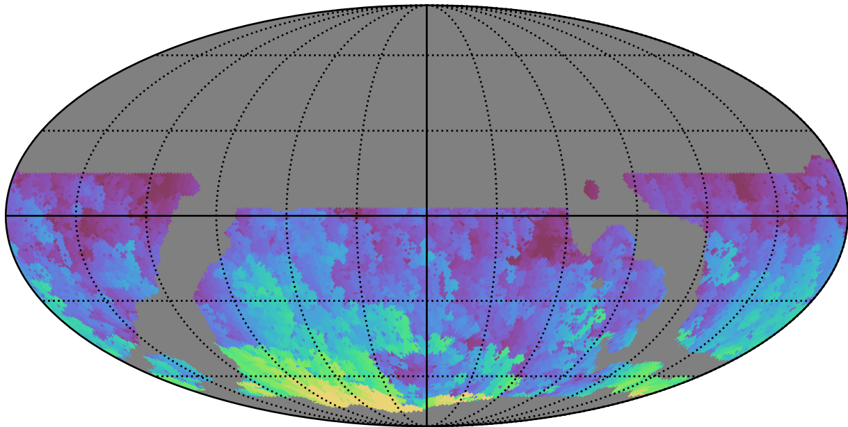
weather_cloudso4v3.4_10yrs WFD g band: Max HA
