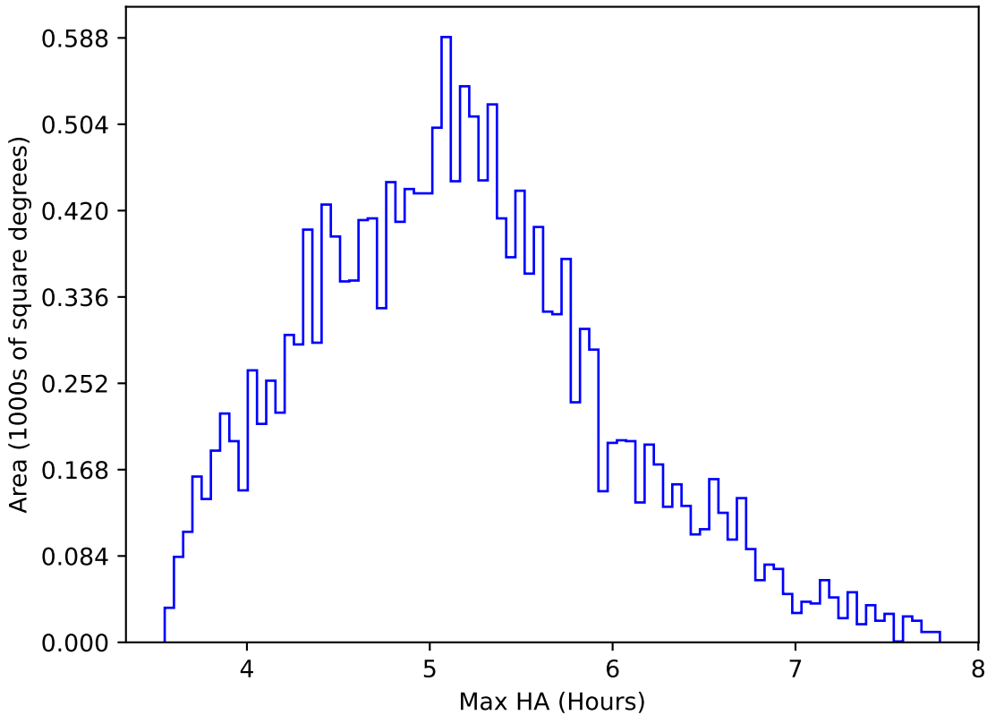
weather_cloudso4v3.4_10yrs WFD all bands: Max HA
