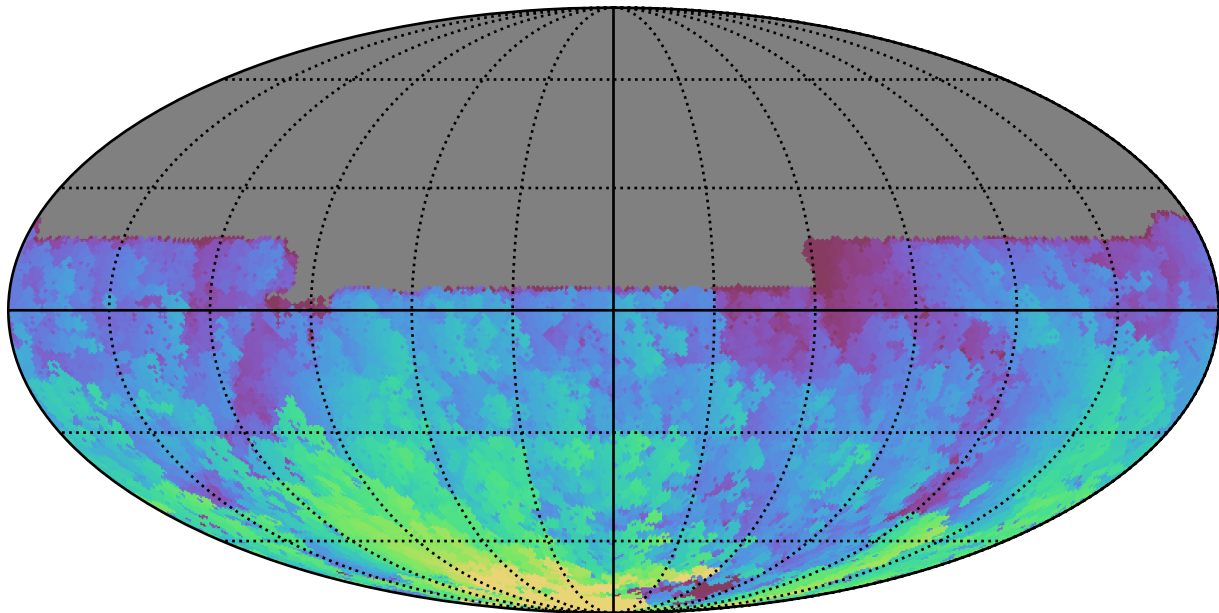
weather_cloudso4v3.4_10yrs All sky u band: Max HA
