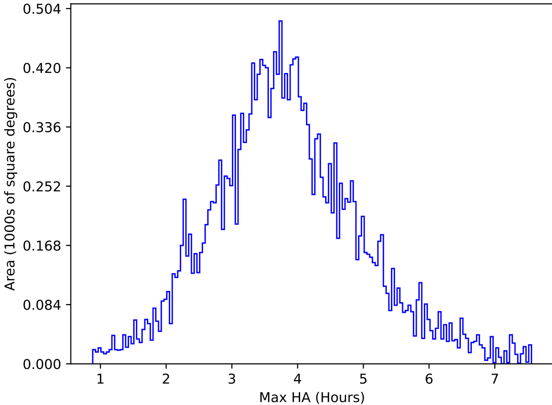
weather_cloudso4v3.4_10yrs All sky u band: Max HA
