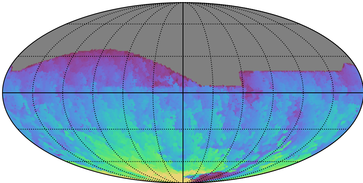
weather_cloudso4v3.4_10yrs All sky r band: Max HA
