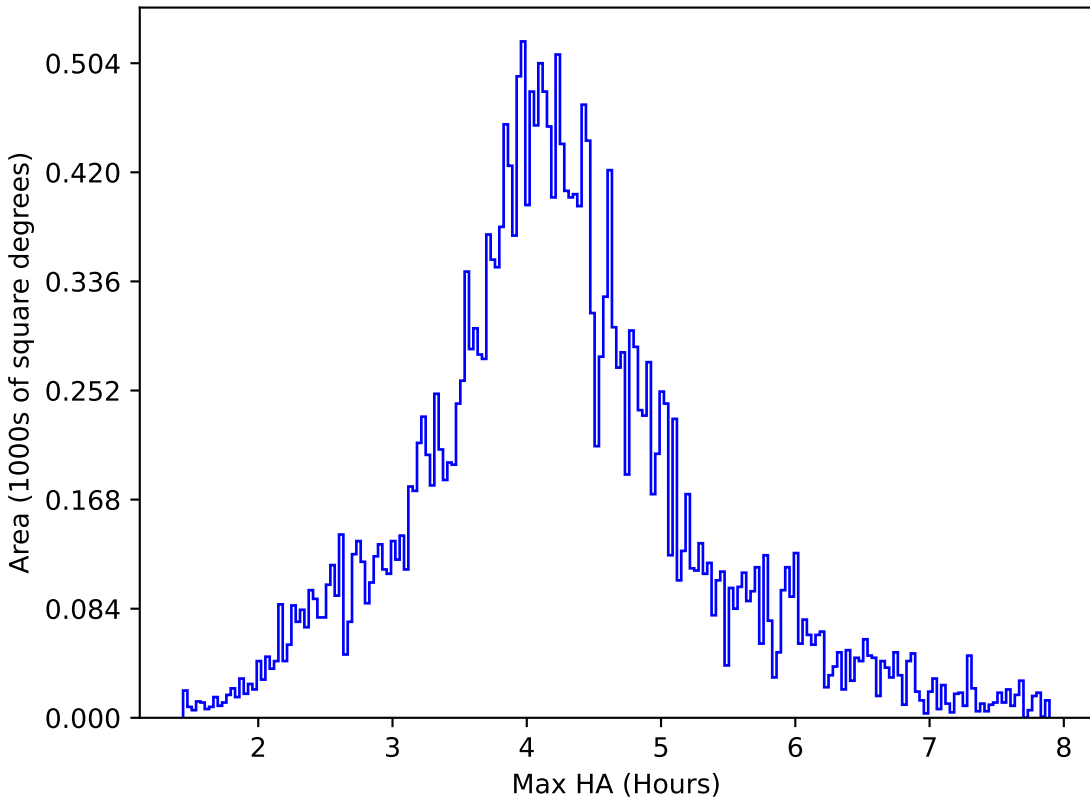
weather_cloudso4v3.4_10yrs All sky r band: Max HA
